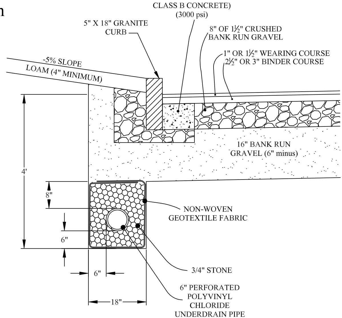
Road Section
