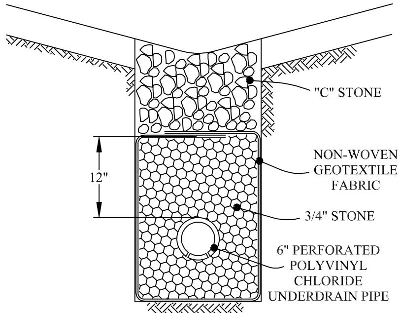
Ditch Section
